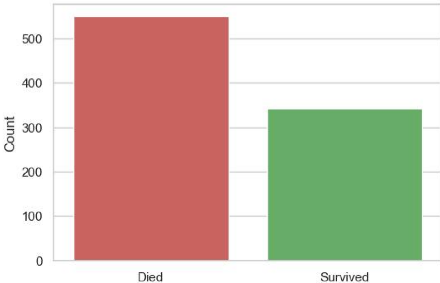
Titanic: Overall Survival Count
