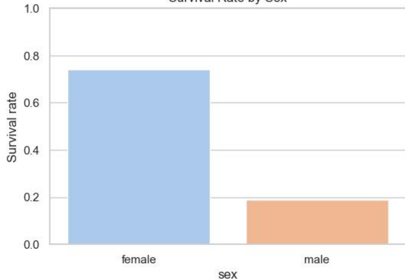
Survival Rate by Sex
