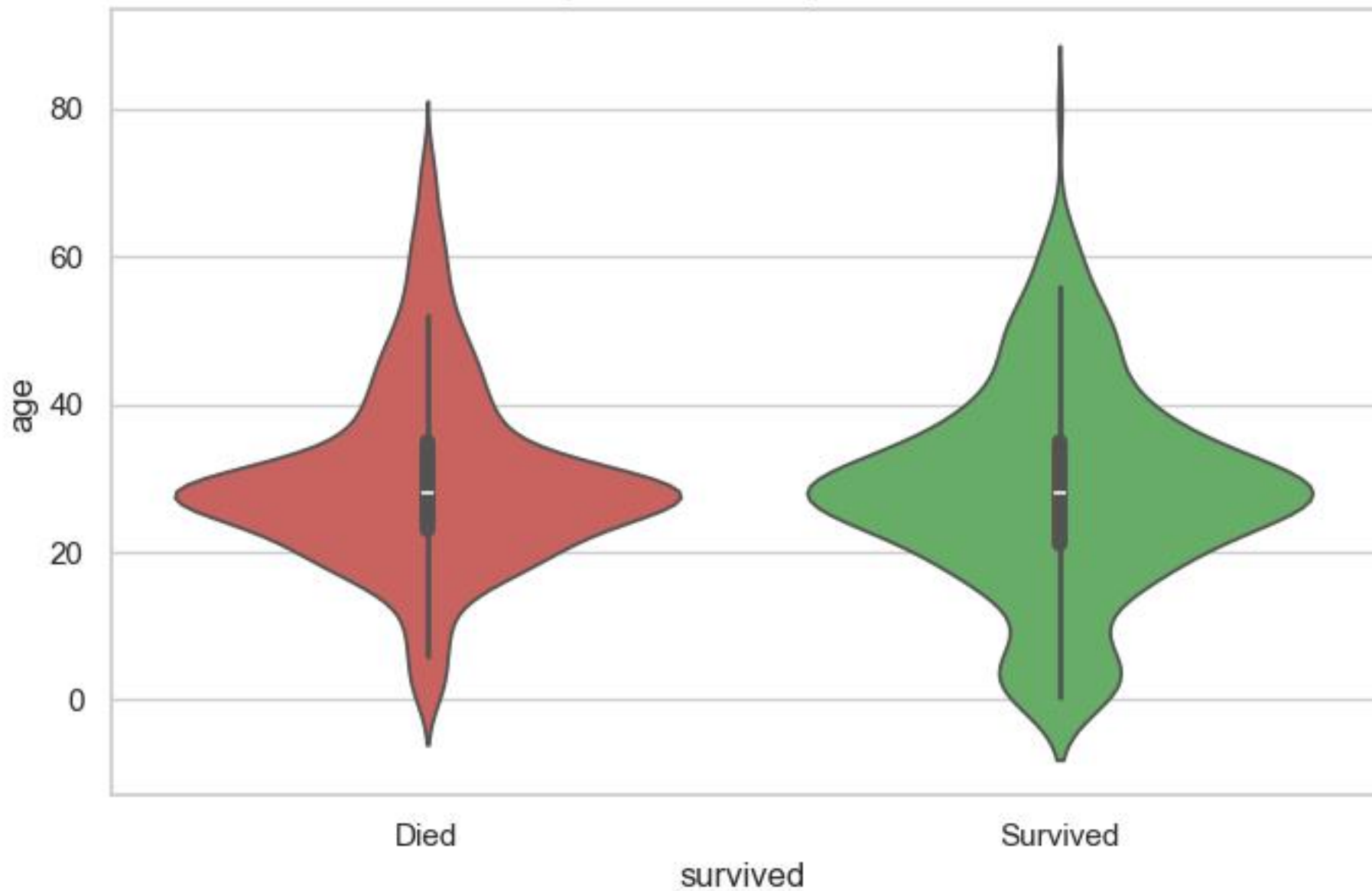
Age Distribution by Survival
